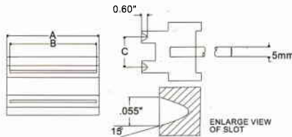
TEMP. CONTROLLED SO DER POT AL400 and DESOLDERING HEAD
